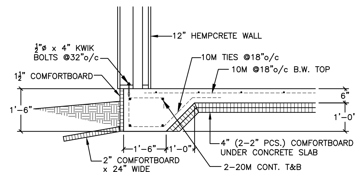
FTN824A: THICKENED EDGE DETAIL *HEATED SLAB RESIDENCE WITH HRV *ALL CONCRETE TO BE 32 MPA CONCRETE. *6" COMPACTED GRAVEL UNDER SLAB
