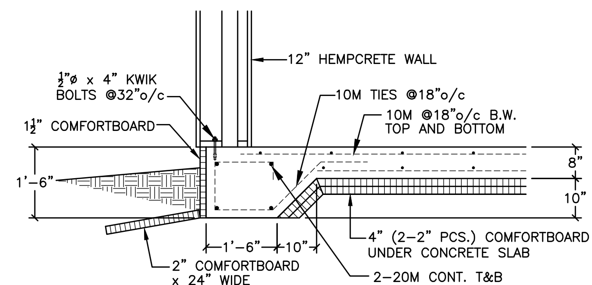
FTN824B: THICKENED EDGE DETAIL *HEATED SLAB RESIDENCE WITH HRV (AT POOL LOCATION ONLY) *ALL CONCRETE TO BE 32 MPA CONCRETE. *6" MIN. COMPACTED GRAVEL UNDER SLAB
